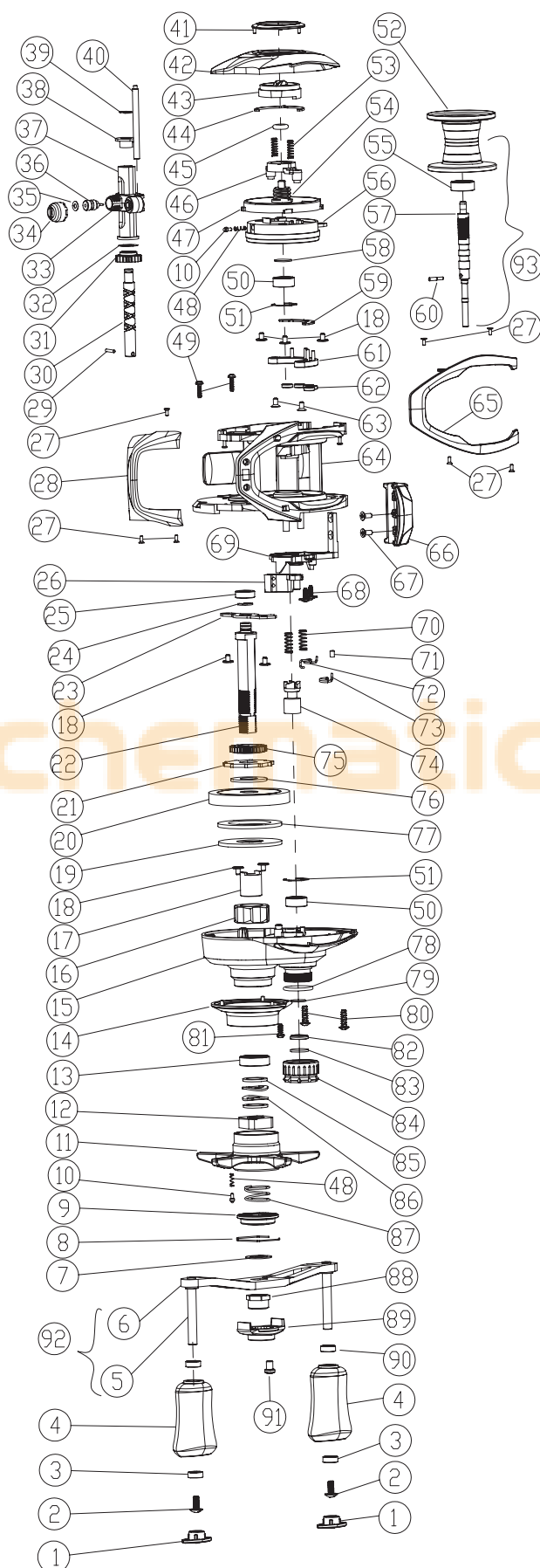
EXPLODED VIEW OF CB5-L66 & CB5R-L66
